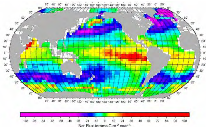
Figure 13: Mean annual sea-air CO 2 flux for the year, 2000 (non-El Nino conditions)
